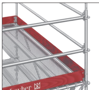
Fig. 52: Corner fitting of toe boards
