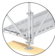
Fig. 95: Base plate fastening with wedge head
