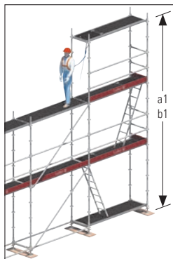
Fig. 12: Attachment overhead
