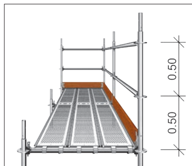
Fig. 19: Three-part side protection in Allround Scaffolding
