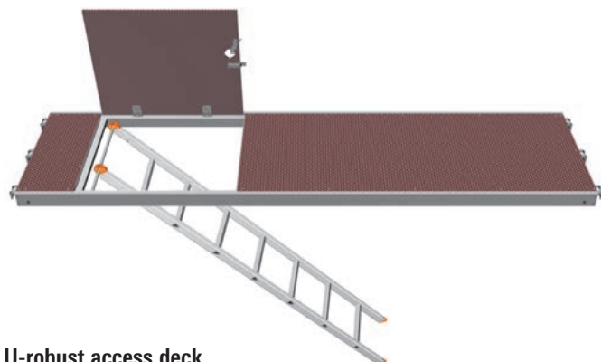
U-robust access deck, 0.61 m wide with integrated access ladder*, access hatch side-opening Ref. No. 3859.xxx, 2.57 – 3.07 m
