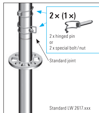
Fig. 88a: Tensile joint with LW standard
