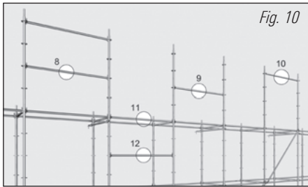
Fig. 9: Attachment in large and small hole of rosette possible (Only permissible in Allround Scaffolding in steel – not in Allround Scaffolding in aluminium) Fig. 10: Attachment points to Allround O- / U-ledgers; maximum bay length 3.07 m
