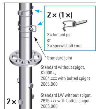
Fig. 88b: Tensile joint with bolted spigot
